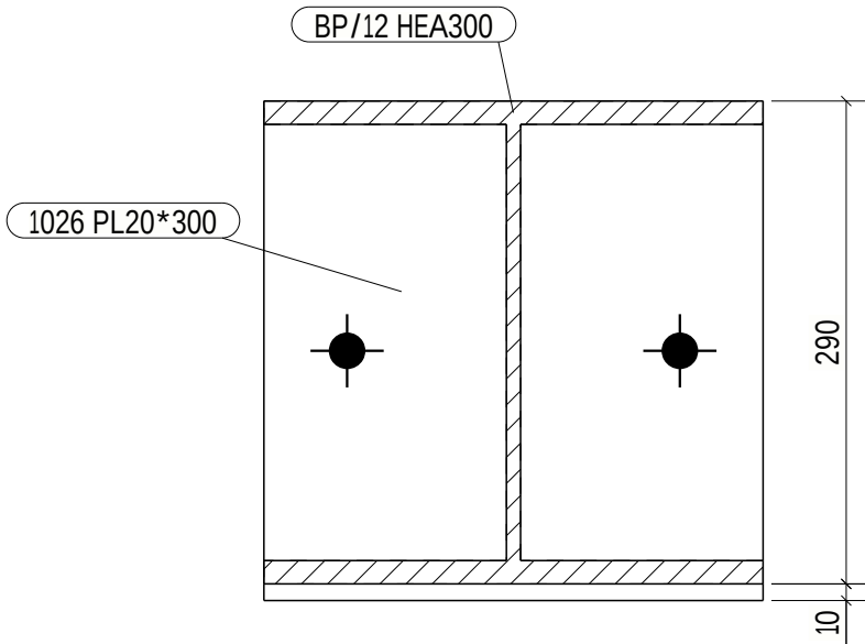
A - A 1:5
